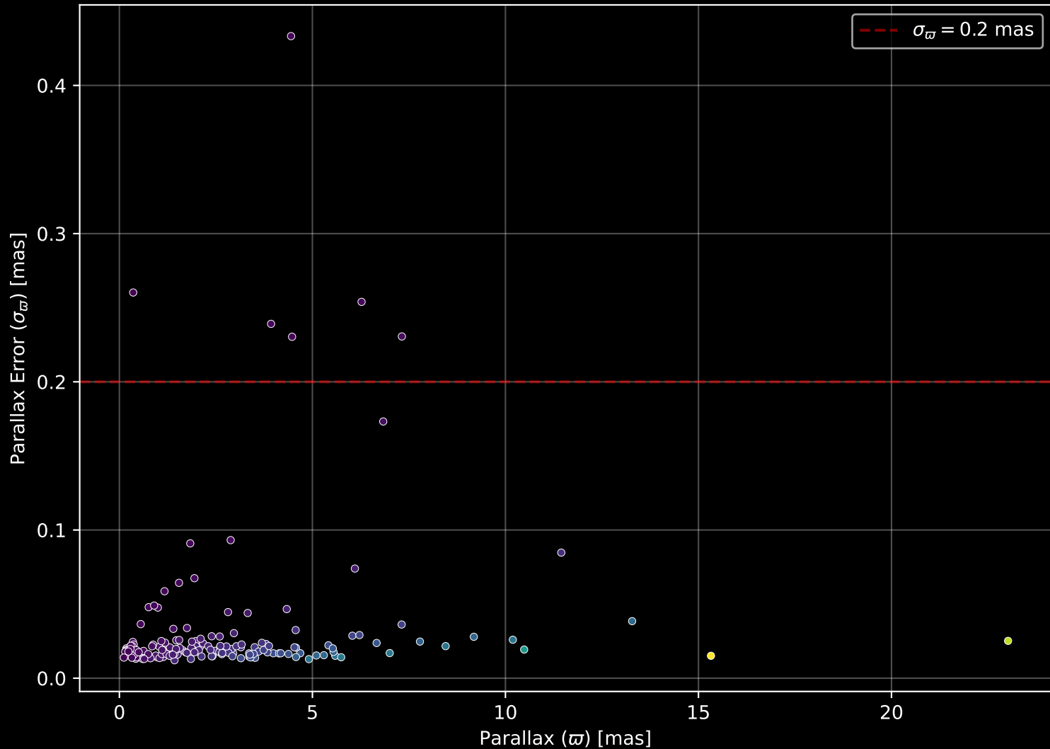
APOGEE DR17 Field: [051-31_MGA] Parallax Quality (n= 168)
