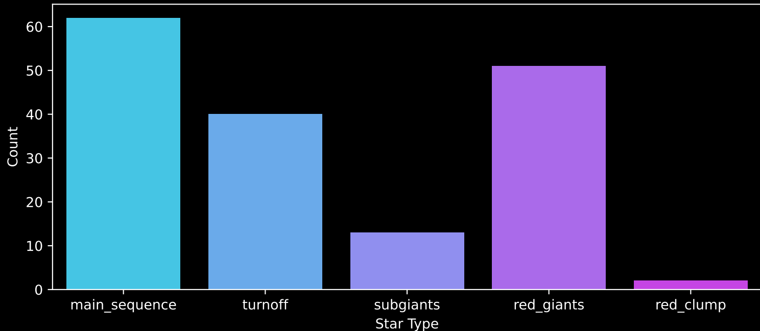
APOGEE DR17 Field: [051-31_MGA] Count plot of Star Type
