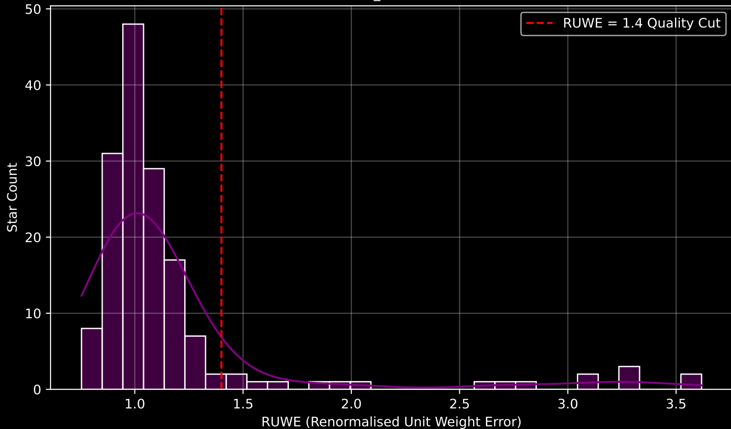
GAPOGEE DR17 Field [051-31_MGA] RUWE Distribution (n= 159)
