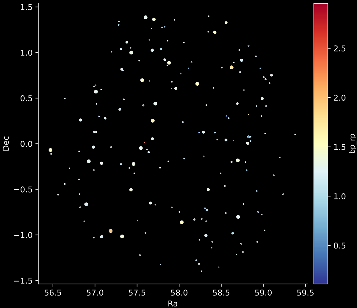
APOGEE DR17 Field: [051-31_MGA] Stars: 168
