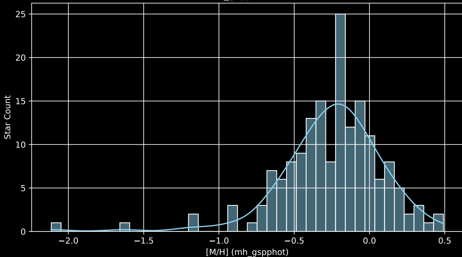
APOGEE DR17 Field: [051-31_MGA [M/H] (mh_gspphot) (n= 167)
