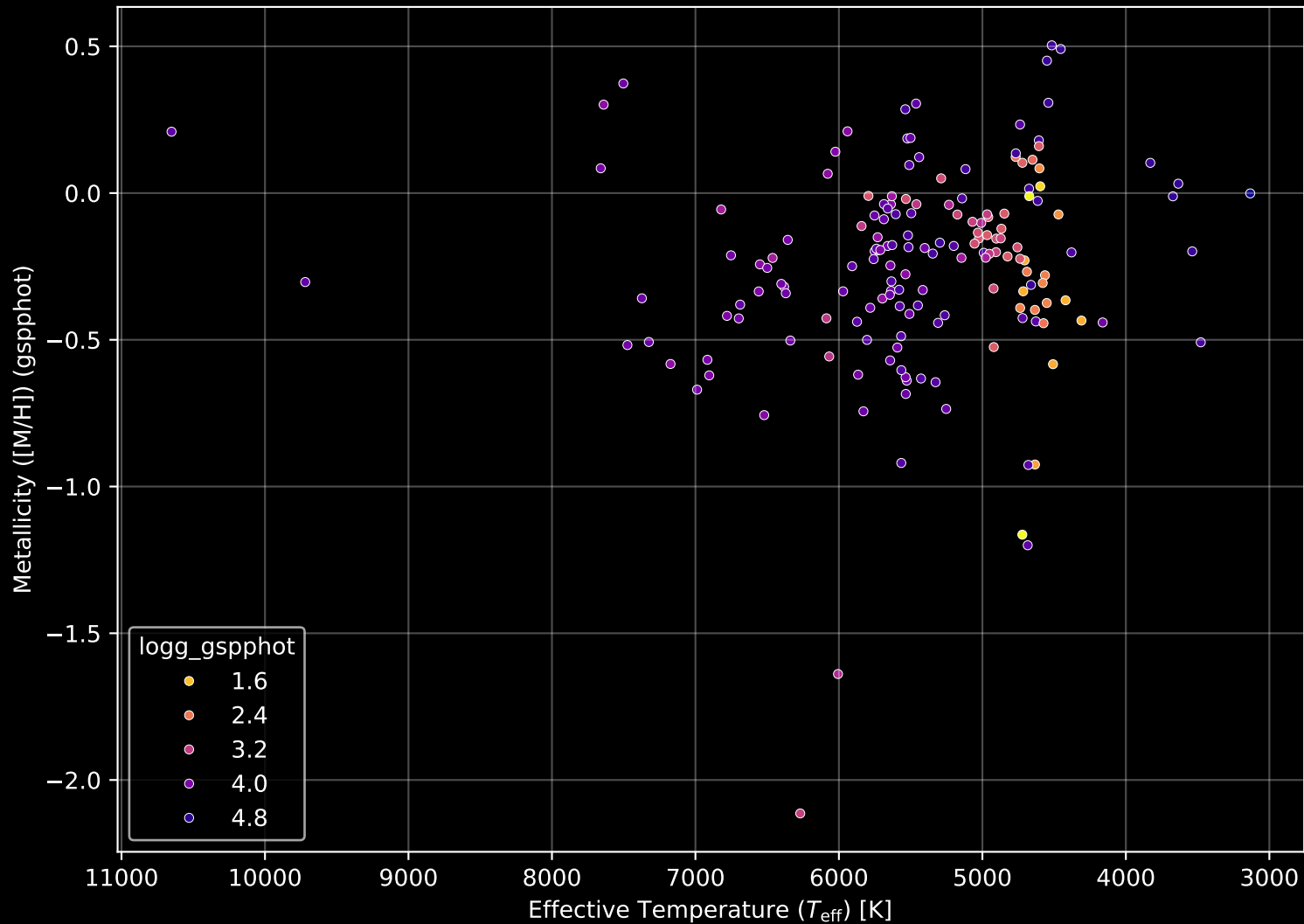
APOGEE DR17 Field: [051-31_MGA] Stellar Population Parameters (n= 168)
