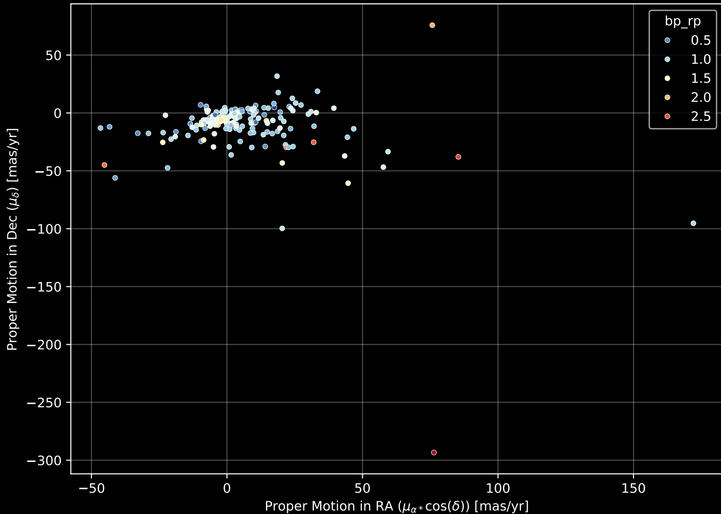
APOGEE DR17 Field: [051-31_MGA] Proper Motion Diagram (n= 168)
